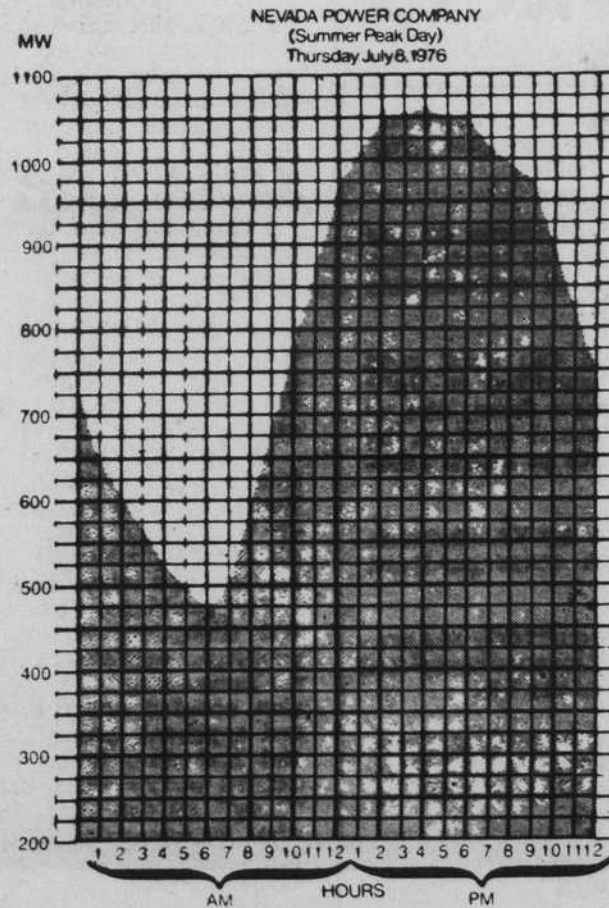
This chart shows how much power was used throughout the day of July 8, 1976 when Nevada Power Company's customers set a new record for power usage. It is called the daily "load curve." You can see how the demand for electricity started climbing about noon to its peak at 4:00 P.M. and then held until about 9:00 P.M. before it slackened significantly. These hours — noon 'til 9:00 P.M. — are "peak hours," the time when our generators are delivering their maximum.
