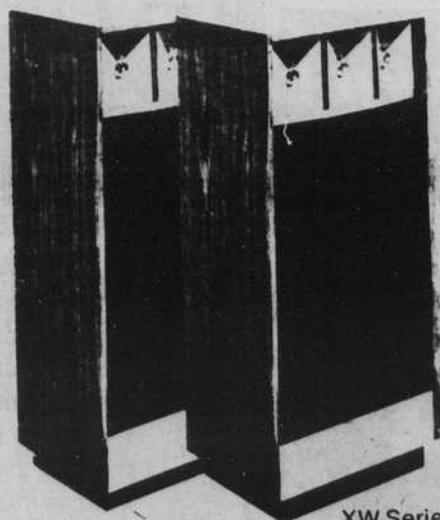
XW Series 24-Speaker Air-Suspension enclosures. Each features a 10" high compliance "duocone" woofer, a 5 1/4" hard back mid-range speaker, three 2" hard back tweeters. Walnut finish cabinets are 36" H x 15 1/2" W x 13" D.
