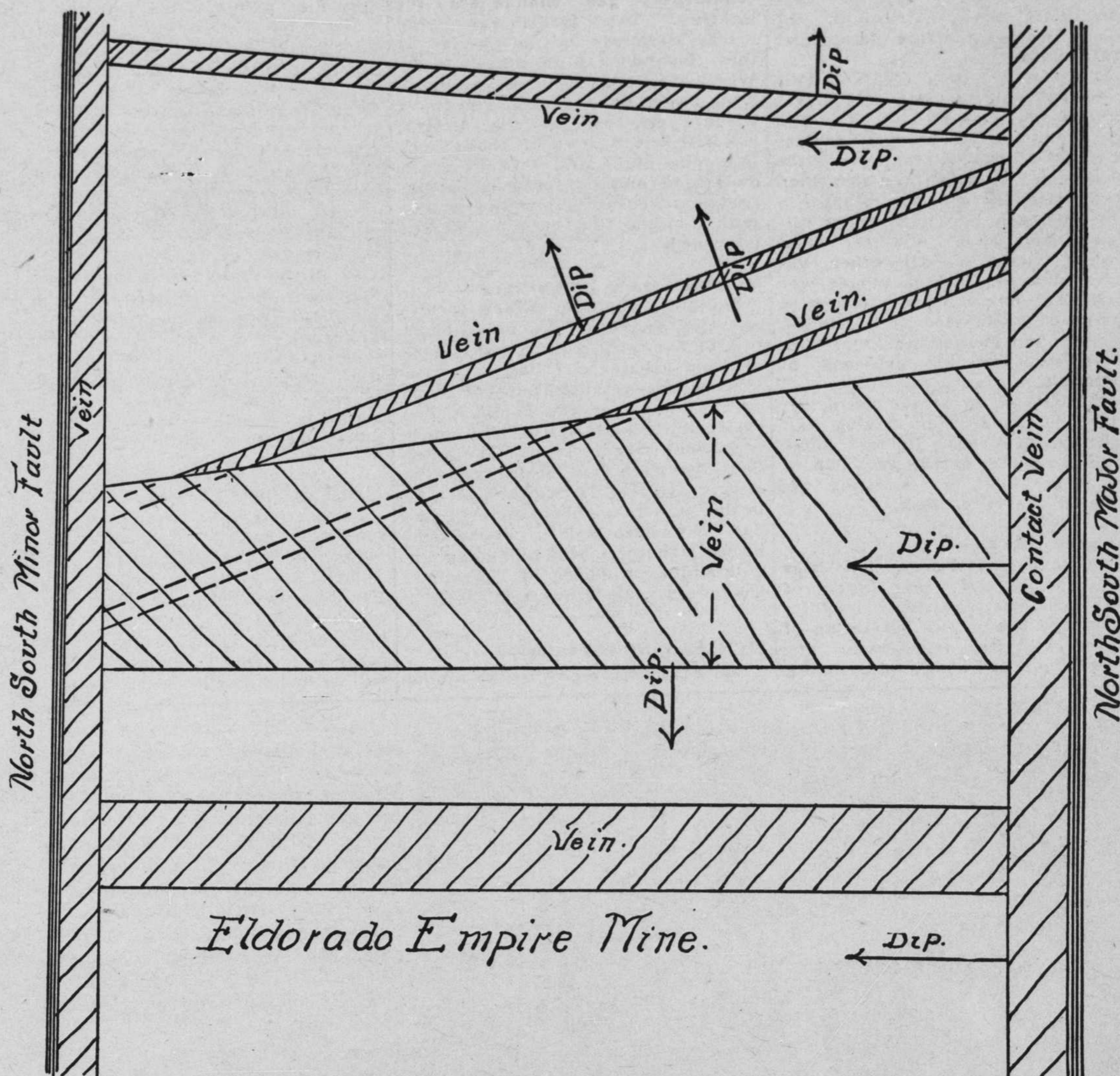
Five East-West ore-filled fractures that meet the North - South Major Fault Vein shown on second sketch.
