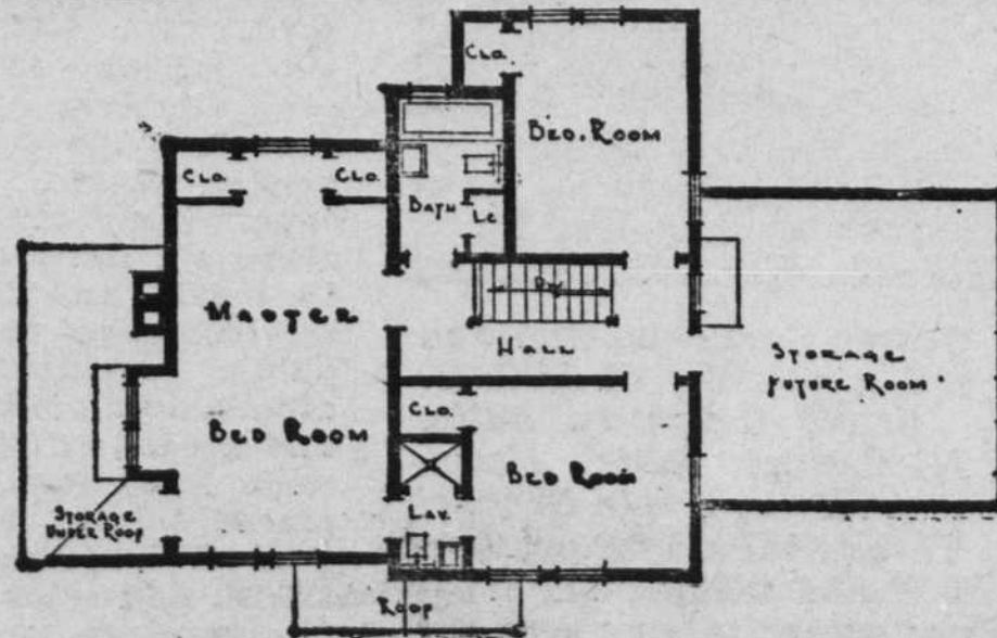
SCALE 1" = 4'-0" SECOND FLOOR PLAN
