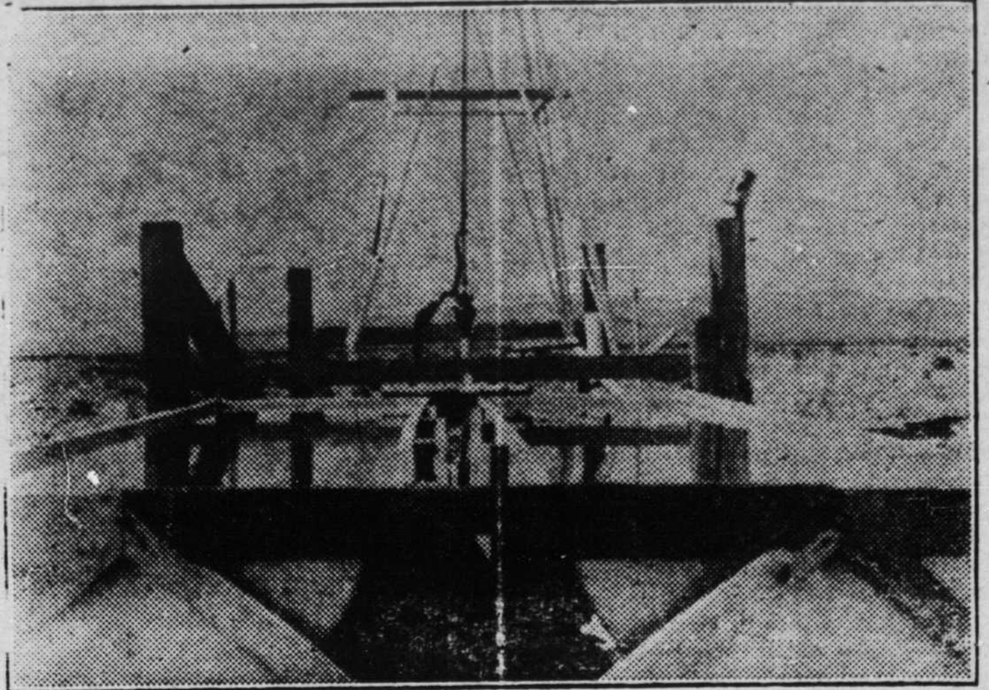
Although being typical as a full Aeromotor windmill operation, this particular object is unusual in the manner in which the troughs were set.
