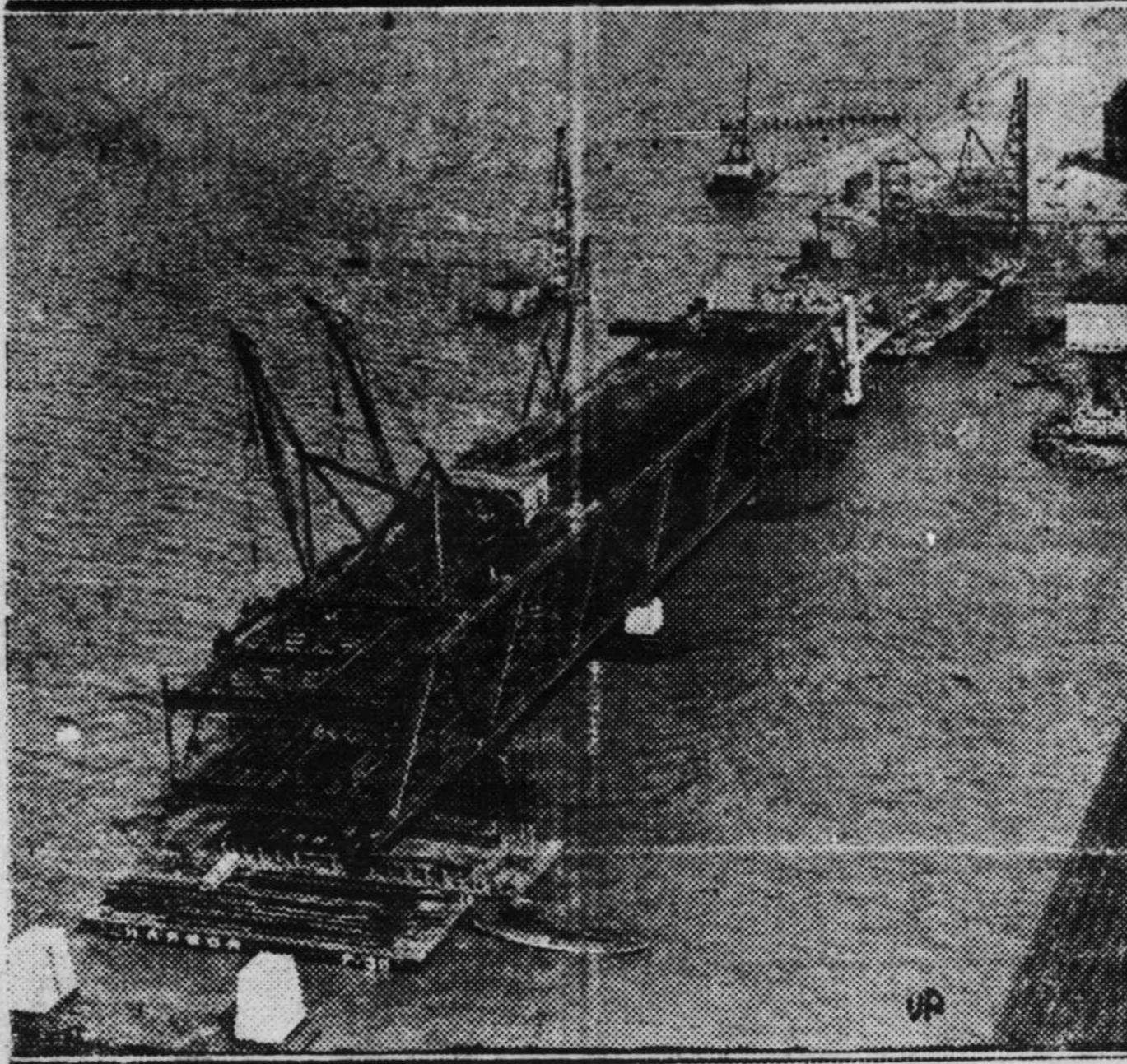
View of the extreme eastern end of the San Francisco-Oakland bay bridge showing traveler derrick with two 87-foot booms erecting the second 288-foot span of the bridge.
