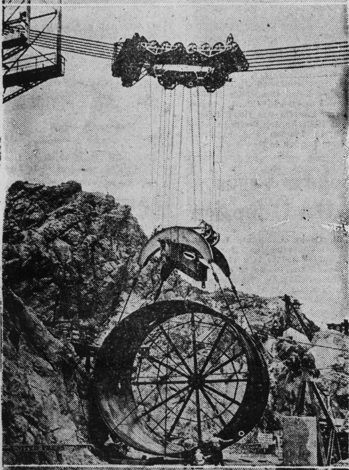
The largest section of steel pipe ever fabricated for an engineering project was placed in final position in the upper Nevada intake tower of the Boulder Canyon project recently, marking another step in the construction of the great Boulder Dam. The pipe is 30 feet in diameter, 21 feet long and weighs 90 tons.
