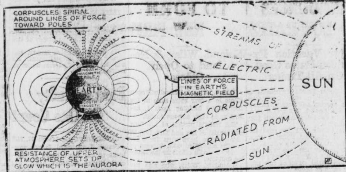
This diagram illustrates how streams of electric corpuscles from the sun, according to the theory of Prof. Carl Stormer, Norwegian scientist, causes resistance in upper atmosphere, creating the 'northern lights'.
