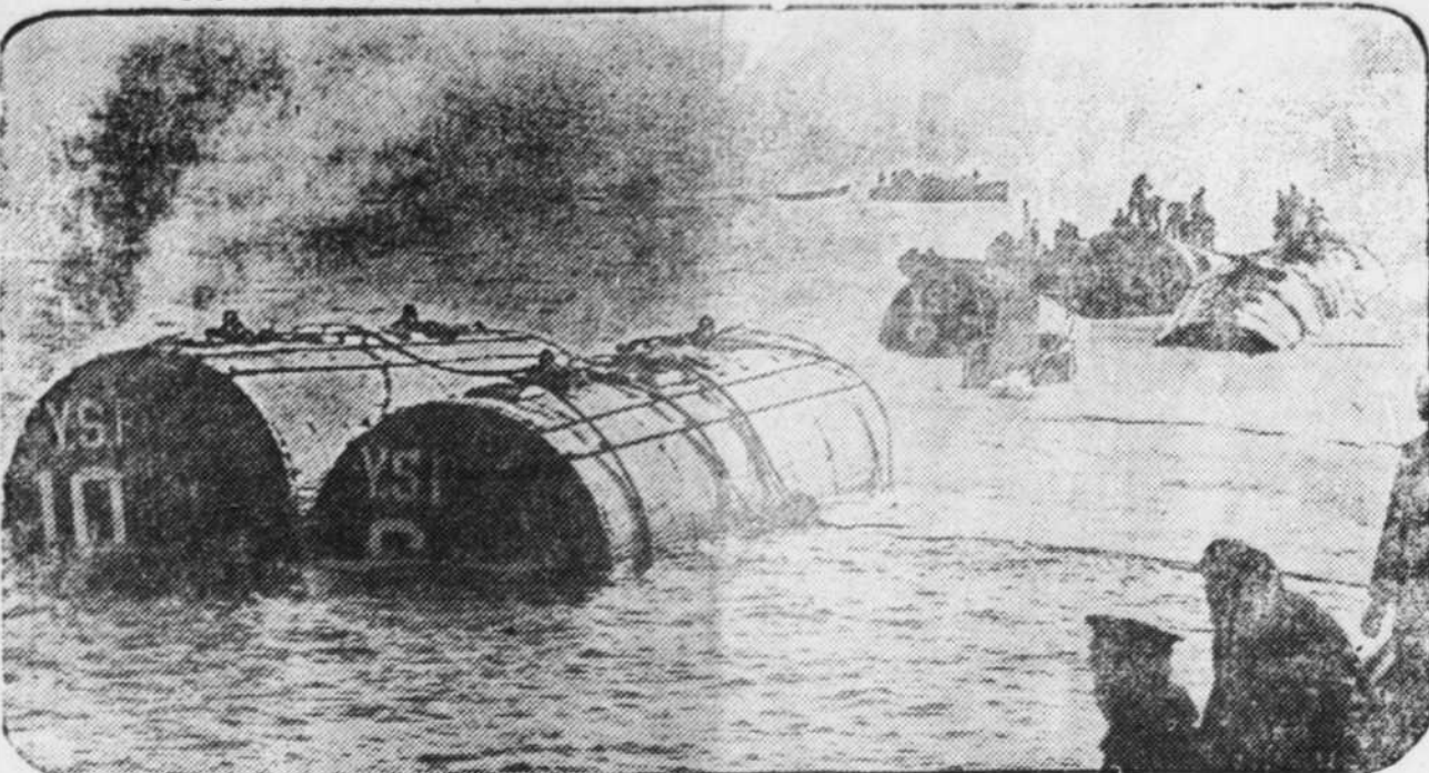
Three months after being rammed by the destroyer Paulding, off Provincetown, Mass., the ill-fated S-4 was brought to the surface, as the picture shows, by six huge air-filled pontoons and towed to the Boston navy yard. The conning tower of the vessel is visible between the cylindrical pontoons.
